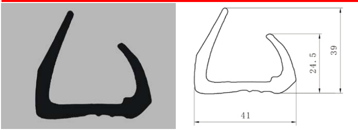
Part No: 072017 Material: Rubber Weight: 0.518KG/M Color: Black
