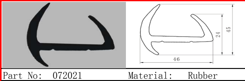
Part No: 072021 Material: Rubber Weight: 0.586KG/M Color: Black
