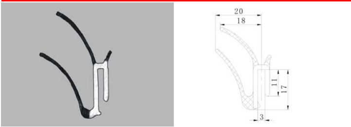
Part No: 072013 Material: Plastic Weight: 0.42KG/M Color: Black&Gray
