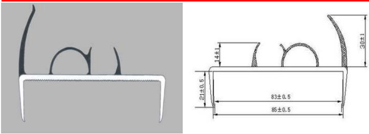
Part No: 072011 Material: Plastic Weight: 0.695KG/M Color: Black&Gray
