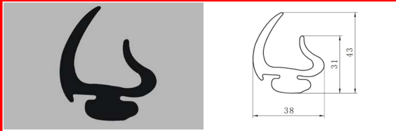
Part No: 072014 Material: Rubber Weight: 0.653KG/M Color: Black
