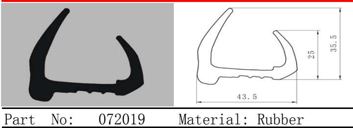
Part No: 072019 Material: Rubber Weight: 0.539KG/M Color: Black
