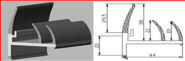
Part No: 072012 Material: Plastic Weight: 0.526KG/M Color: Black&Gray
