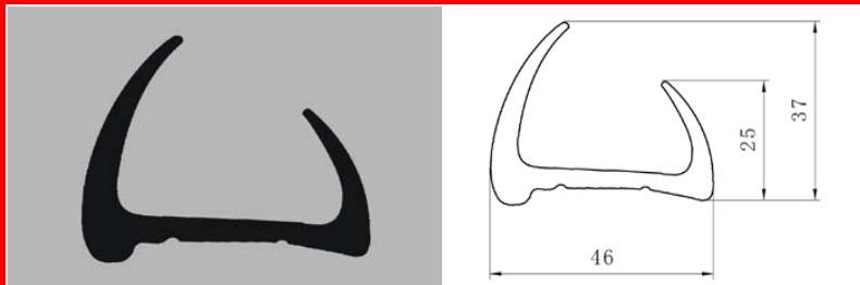
Part No: 072018 Material: Rubber Weight: 0.564KG/M Color: Black
